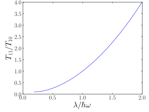
FIG. 3. (Color online) Ratio of elastic and inelastic transmission probabilities in the first vibrationally excited state. At weak coupling, the elastic transmission T_{11} goes to zero indicating that a vibrational excitation results in only a single electron being transmitted.
